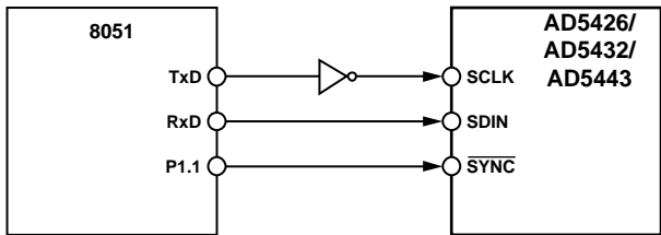
Figure 55. 80C51/80L51-to-AD5426/AD5432/AD5443 Interface
