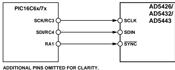
Figure 58. PIC16C6x/7x-to-AD5426/AD5432/AD5443 Interface
