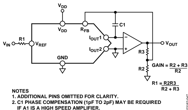
Figure 46. Increasing Gain of Current Output DAC
